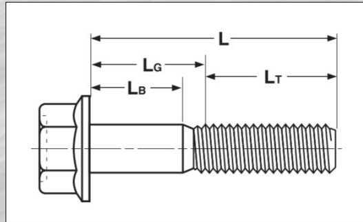
MAXIMUM GRIP GAGING LENGTHS, L, AND MINIMUM BODY LENGTHS, L
